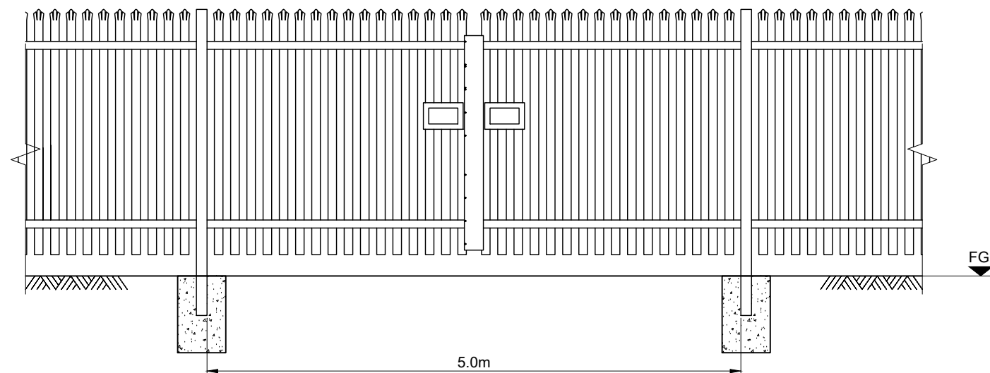
TYPICAL PALISADE FENCE ELEVATION (DOUBLE VEHICLE GATE)
