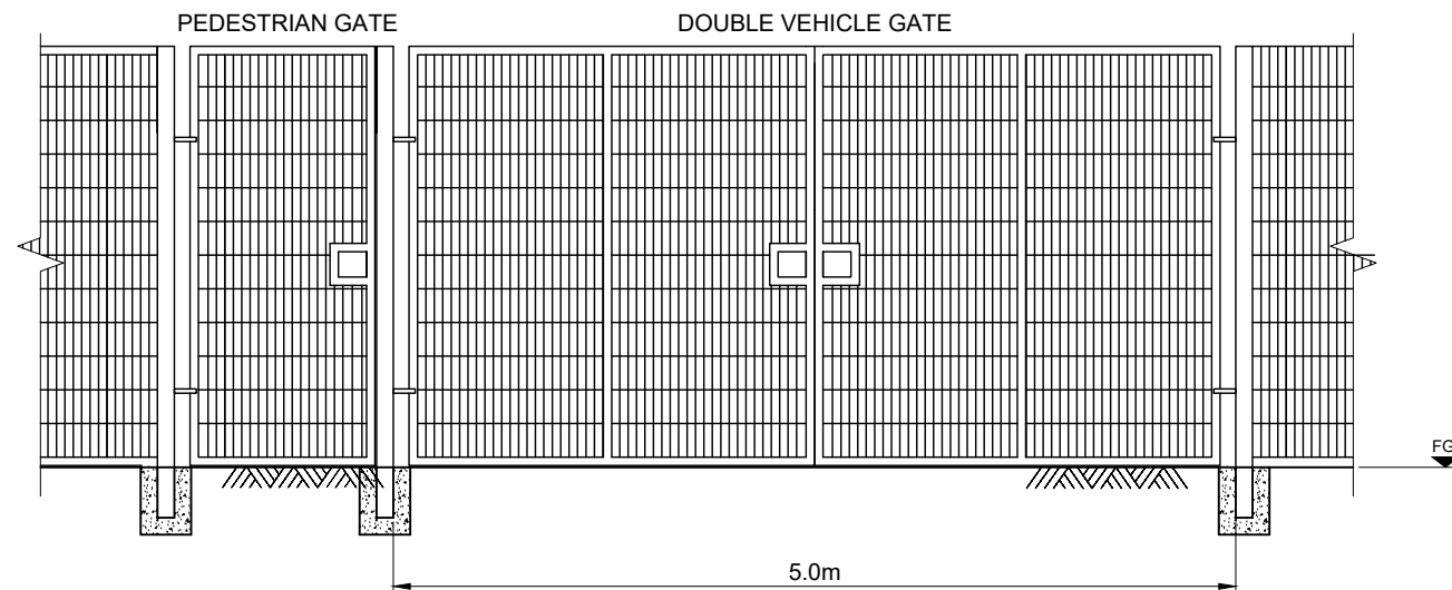
TYPICAL WELD MESH FENCE ELEVATION
