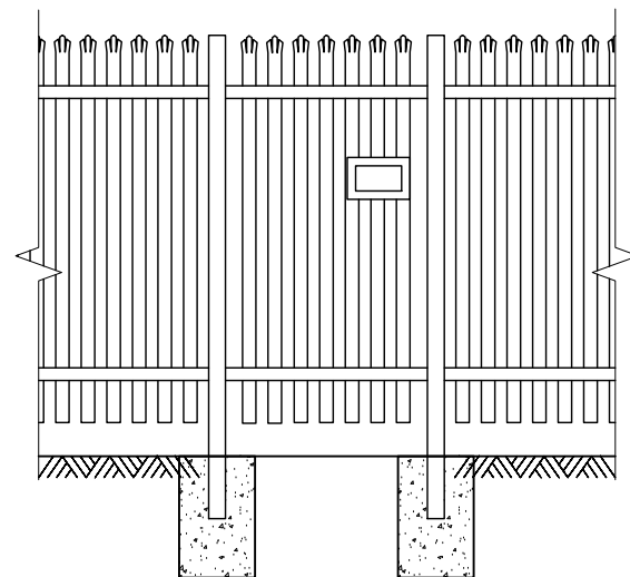
TYPICAL ELEVATION (PEDESTRIAN GATE)
